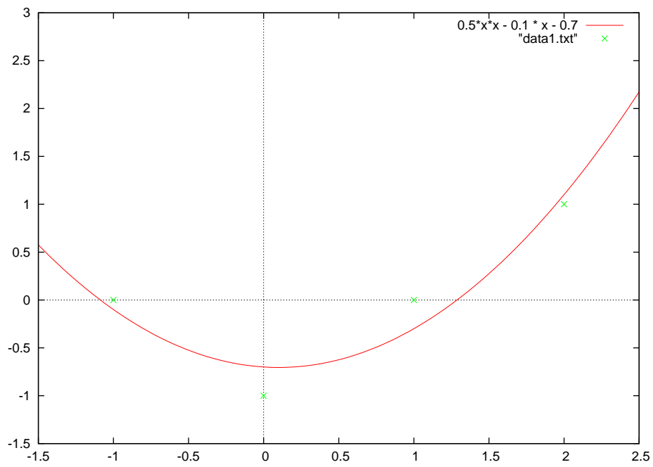
Figure 1: The parabola closest to the given four points
